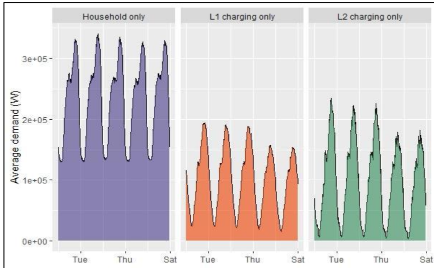
Figure 4.2 "Average yearly power demand on working days"
