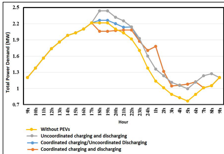
Figure 2.3 "Total power demand in different scenarios (31% market share) [17]"
